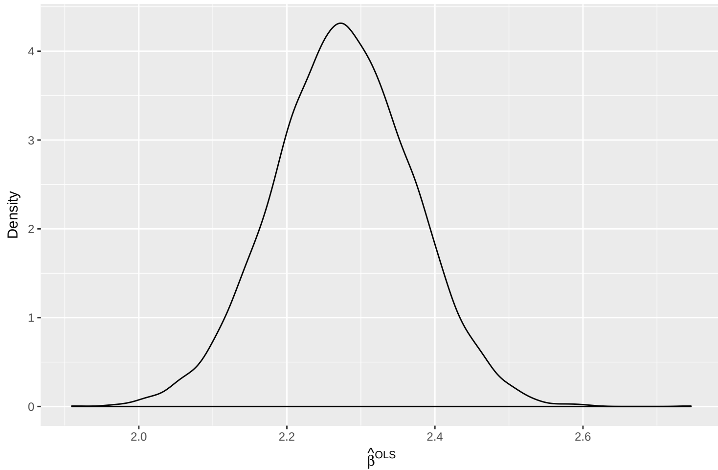
Density of OLS Estimator with N = 100
